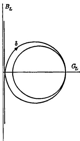
FIG. 16-4.—Admittance curve.
